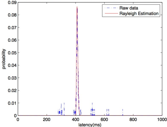
Fitted Sao Paulo Latency (Mobile to Cloud Server via WiFi) Curve using Rayleigh Distribution
