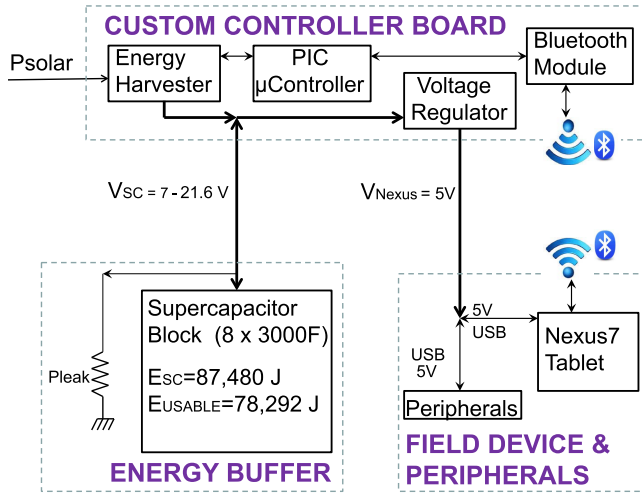
Fig. 2. System architecture including the supercapacitor block for energy buffering, Nexus 7 for energy consumption, and a custom-built 70mW controller board that regulates between solar power input and energy buffering/consumption.
