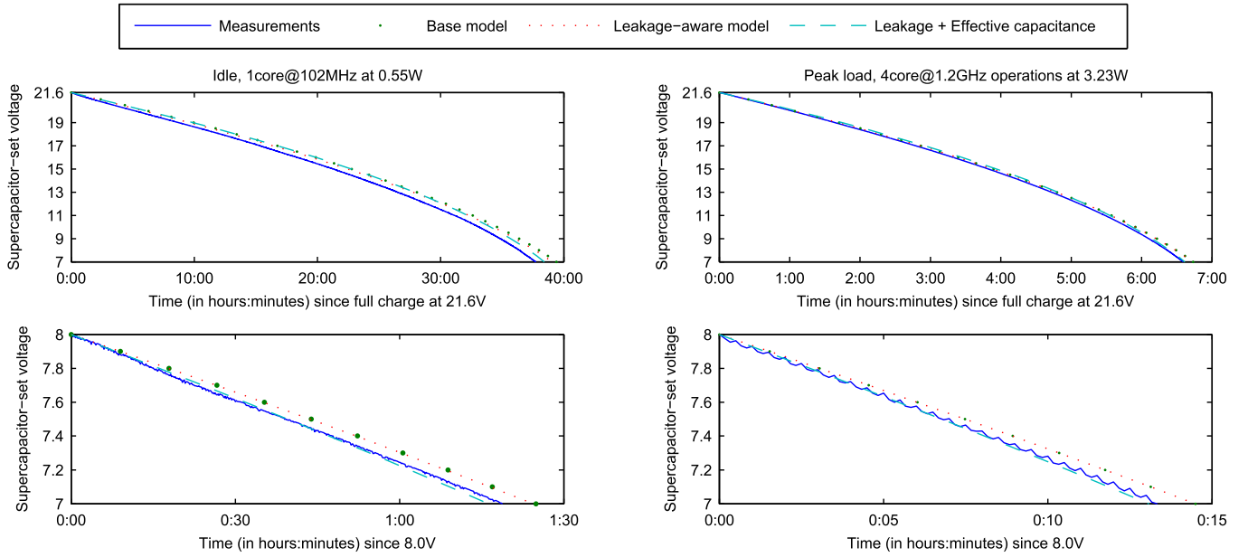
Fig. 7. Time prediction evaluation —Accuracy of different supercapacitor energy models in predicting the time to reach a certain target voltage under specific power loads. The left two plots illustrate the results under idle load while the right two plots show the results under a high-load condition for the ZoneMinder-based environmental camera traps. The top two plots illustrate the results of modeling the operational time from the full charge of 21.6 V for the supercapacitors while the bottom two plots show the results of modeling from 8 V to 7 V.
