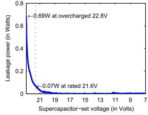
Fig. 4. Self-discharge (leakage) power for our 8-supercapacitor set at operating and overcharged voltages.
