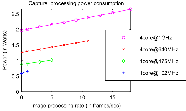
Fig. 6. Data capture+processing power consumption at a range of CPU configurations and application frame rates. For each CPU configuration, the experiments end at the maximum achievable frame rate. We also show a linear fitting of the frame rate to power each CPU configuration.
