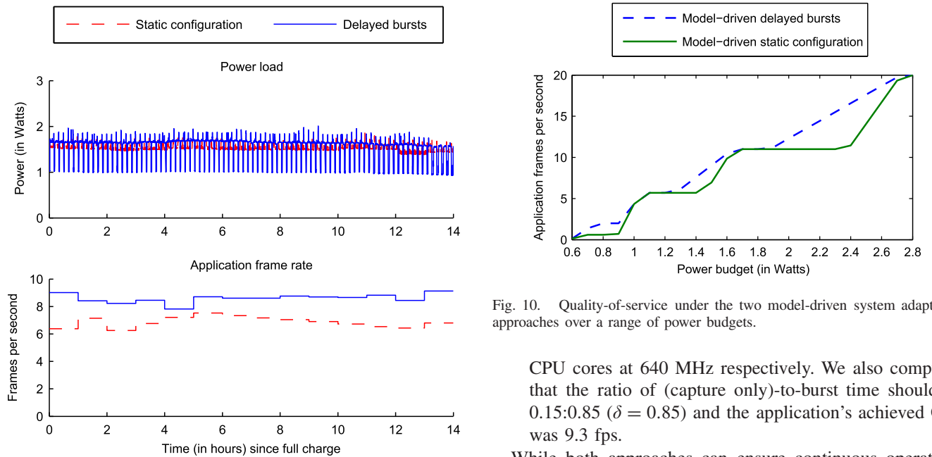
Fig. 9. Power consumption, application frame rate under model-driven static CPU configuration and delayed bursts.
