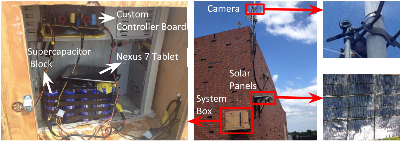
Fig. 1. Deployed system on a seven-story building rooftop (center picture) that includes a camera, a block of solar panels, and a system box. The system box (left-side picture) contains a Nexus 7 tablet computer (without its internal rechargeable battery) sustained by eight Maxwell 3000 Farad supercapacitors (wrapped in black tapes), and a custom-built controller board (at the top of the box). The energy buffering capacity of the supercapacitor block is about 1.4\times that in the original Nexus 7 battery.
