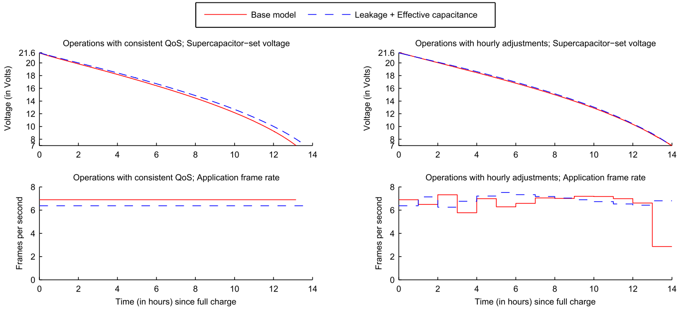
Fig. 8. Power budget evaluation—Effectiveness of supercapacitor energy models in guiding application operational frame rates to utilize the stored energy by a certain amount of time. The experiments were performed for the traffic trajectory analysis application. The left two plots illustrate the supercapacitor voltage and application frame rates under operations of consistent frame rates. The right two plots show the results when the system makes hourly assessment of remaining supercapacitor energy and adjustment of application frame rates.
