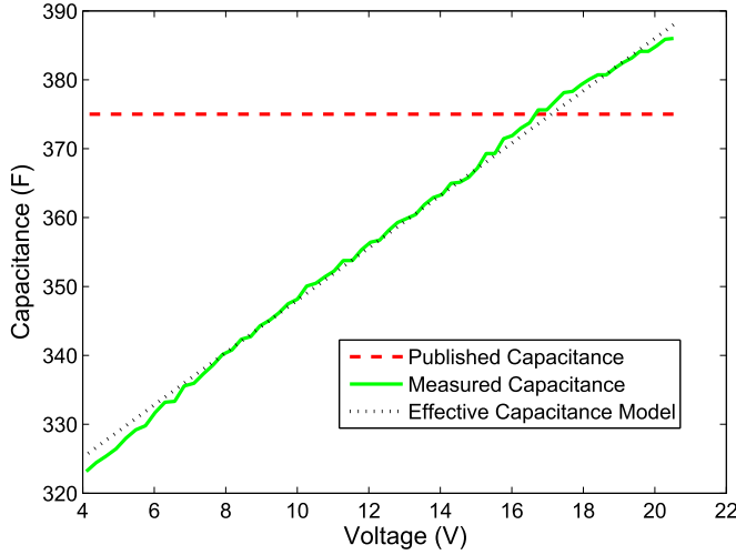
Fig. 5. Effective capacitance at different terminal voltages. The capacitance is noticeably lower at low voltages.
