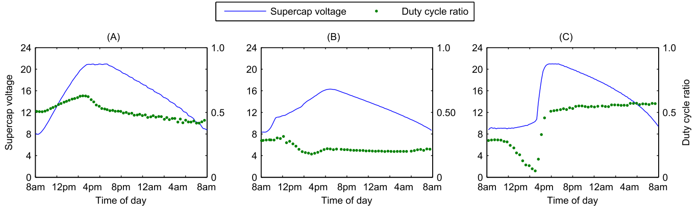
Fig. 11. System duty-cycle ratio and supercapacitor voltage changes in 24-hour periods of our outdoor system deployment under sunny (A), overcast (B) and mixed (C) weather conditions.
