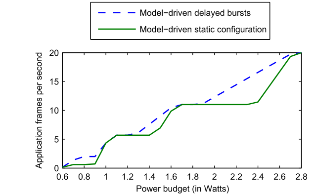
Fig. 10. Quality-of-service under the two model-driven system adaptation approaches over a range of power budgets.
